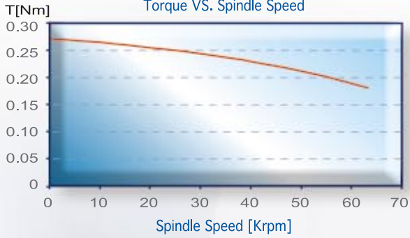
Torque VS. Spindle Speed
