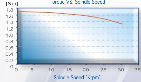
Torque VS. Spindle Speed
