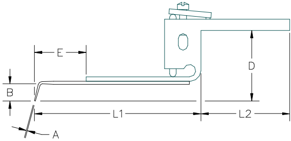
Z-Adjustable Geometry
