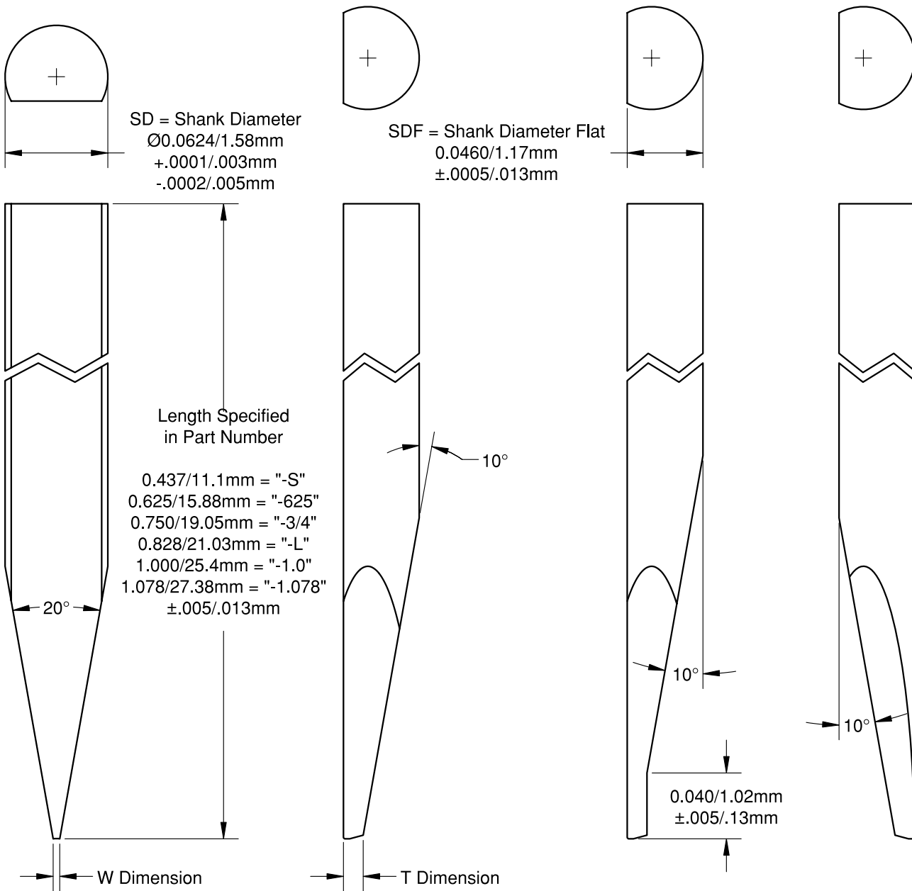
180° Reverse Shank Dias Bonder Models US1800A & US1900A K&S Bonder Models 8060 & 8090 (Not Available on Deep Access, Vertical Feed Style Tools)
